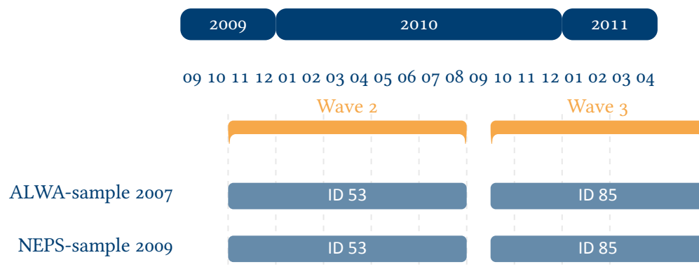
Figure 2: Surveys of Starting Cohort 6 and IDs of the instruments
