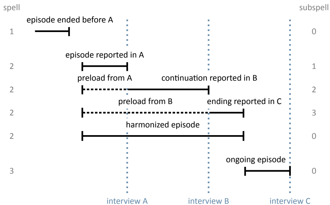
Figure 20: Logic of subsPELL
