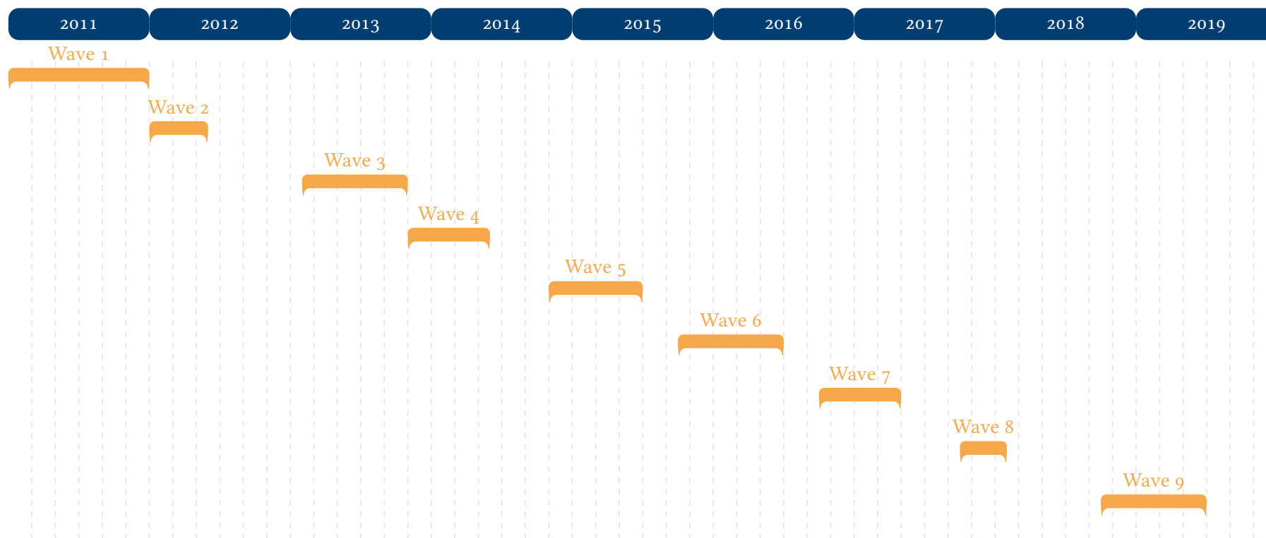
Figure 1: Survey progress of Starting Cohort 2 (waves 1-9)
