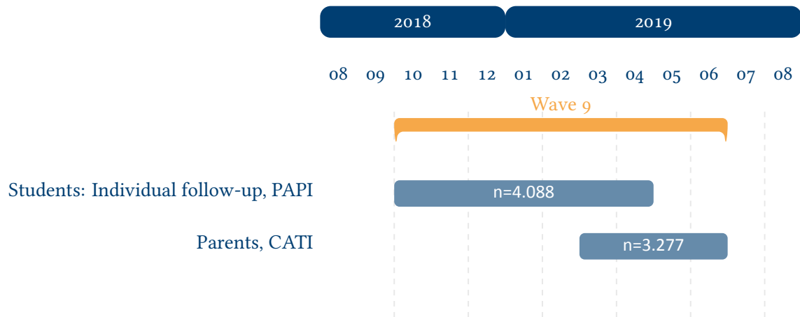
Figure 10: Field times and realized case numbers in wave 9
