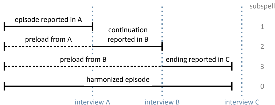
Figure 14: Logic of subsPELLs
